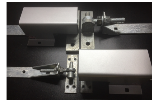
CHOOSE LEFT OR RIGHT OR RIGHT HINGED
